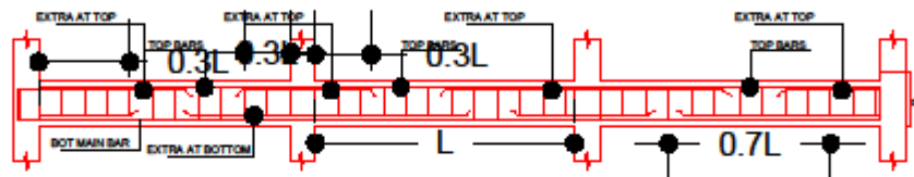
TYPICAL SECTION OF BEAM REINFORCEMENT
