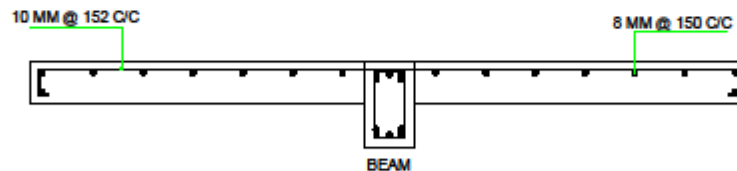
( SLAB 1 ) BEAM SLAB DETAIL (150 MM THK.)
