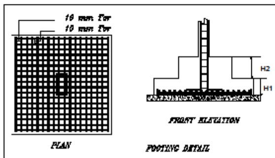
FOOTING DETAIL-F1
