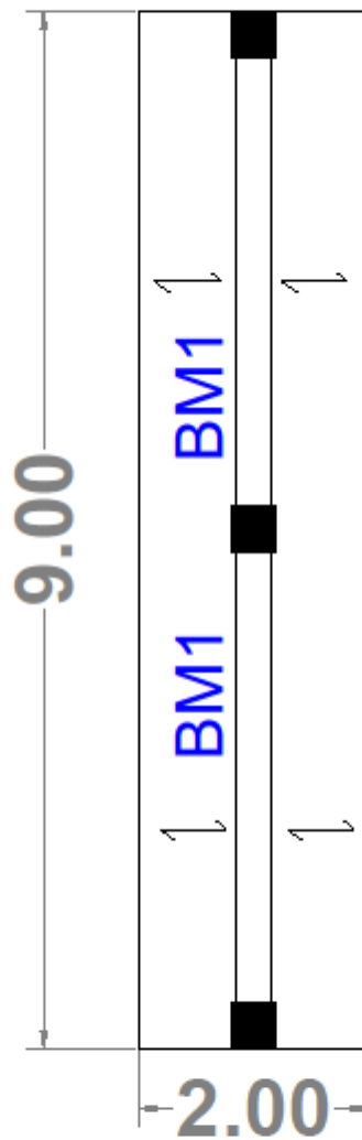
BEAM PLAN+2500 MM LVL
